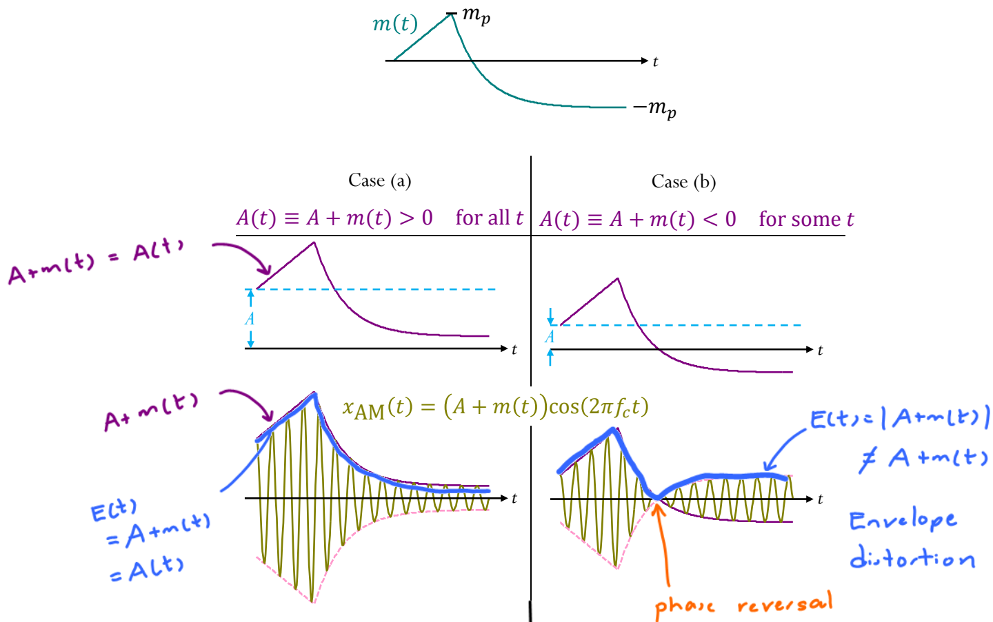
Figure 27: AM signal and its envelope [6, Fig 4.8]
