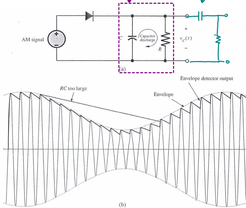
Figure 30: Envelope detector for AM [6, Fig. 4.11].
