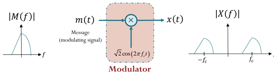
Figure 26: DSB-SC modulation.
