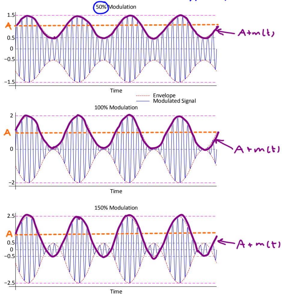
Figure 28: Modulated signal in standard AM with sinusoidal message
